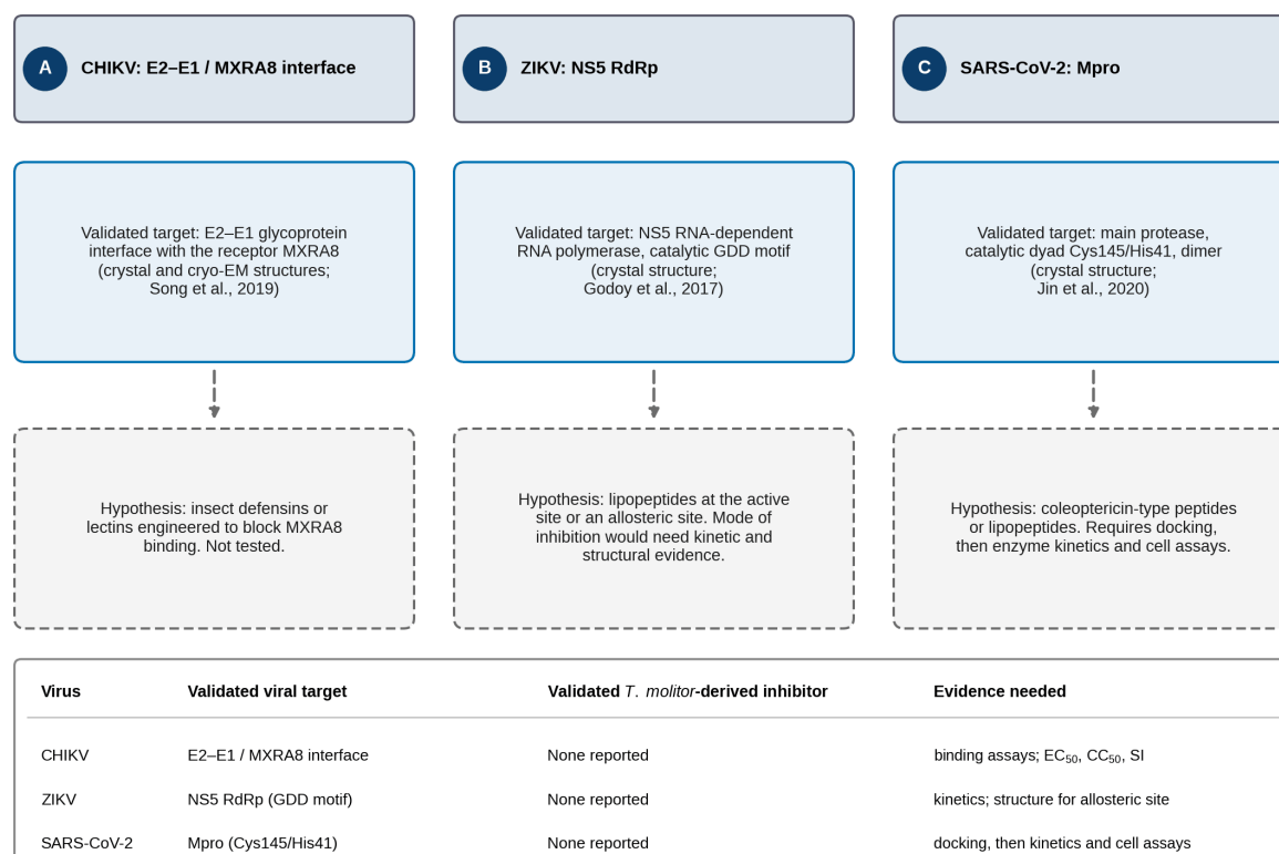
Figure 4: Validated structural viral targets and hypothesized insect-derived inhibitors. Solid blue boxes show viral targets whose structures have been determined experimentally; dashed boxes show hypotheses that have not been tested. (A) CHIKV: the E2–E1 glycoprotein interface with the receptor MXRA8 (Song et al., 2019); blockade by insect defensins or lectins is a hypothesis. (B) ZIKV: the NS5 RdRp and its catalytic GDD motif (Godoy et al., 2017); inhibition by lipopeptides has not been reported, and a competitive or allosteric mode would require kinetic and structural evidence. (C) SARS-CoV-2: the main protease Mpro, with catalytic dyad Cys145/His41 (Jin et al., 2020); an effect of coleopteracin-type peptides or lipopeptides is a hypothesis that requires docking followed by enzyme kinetics and cell-based assays. The summary table separates validated viral targets from validated T. molitor -derived inhibitors, for which none has been reported. RdRp, RNA-dependent RNA polymerase; SI, selectivity index.
